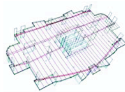
3D FEM Models of Slab Showing Tendons, Deflection and Shop Drawing
