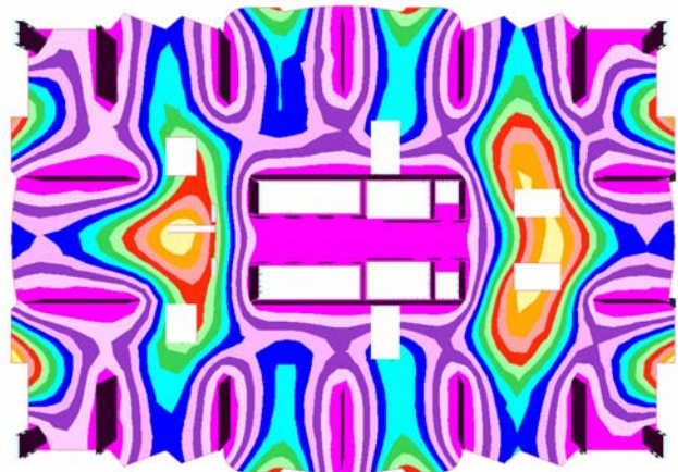
Deflection Contour from FEM Analysis
