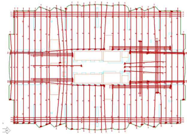
3D Tendon Model of PT Flat Slab
